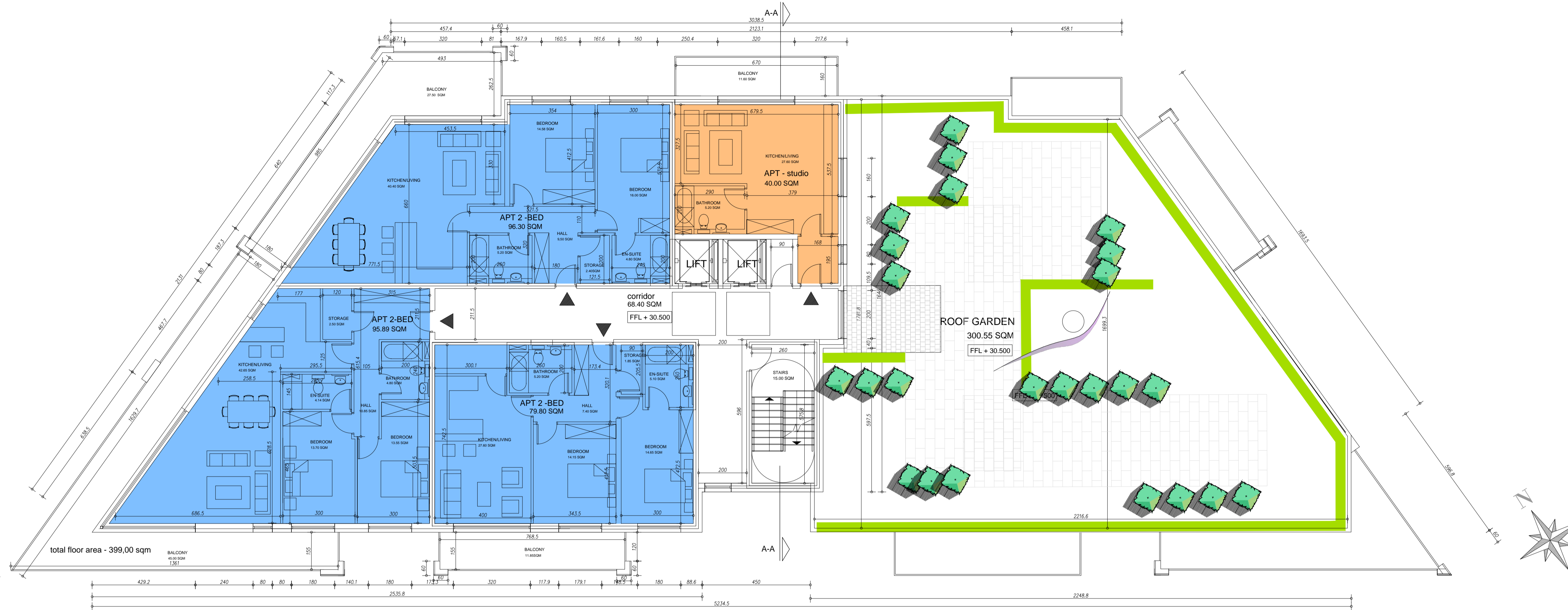
1 PROPOSED BLOCK 2 - PENTHOUSE - 8-TH FLOOR PLAN 1 : 100
